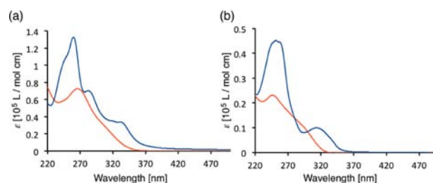
Figure 4. Absorption spectra of (a) cyclophane 1c (blue) and 4c (red) and (b) clipped structure 2b (blue) and 5b (red) in THF ( [c] = 5.0 \times 10^{-6} \text{ M} ).
