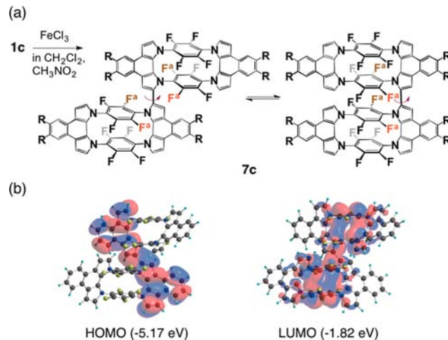
Scheme 2. (a) Synthesis and Conformational Equilibrium of Cyclophane Dimer 7c and (b) the Frontier MOs for the DFT-Optimized Structure at the B3LYP/6-31G(d) Level of Theory
