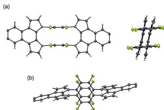
Figure 3. Crystal structure of cyclophane 1b : (a) side views and (b) top view. Thermal ellipsoids are at 50% probability, and alkyl chains are omitted for clarity.
