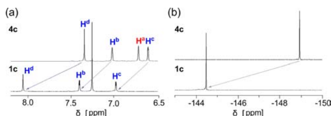
Figure 2. (a) ^1\text{H} and (b) ^{19}\text{F} NMR spectra of 1c and 4c in \text{CDCl}_3 .
