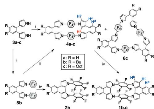
Scheme 1. Synthesis of Paracyclophane 1 and Clipped Structure 2'
