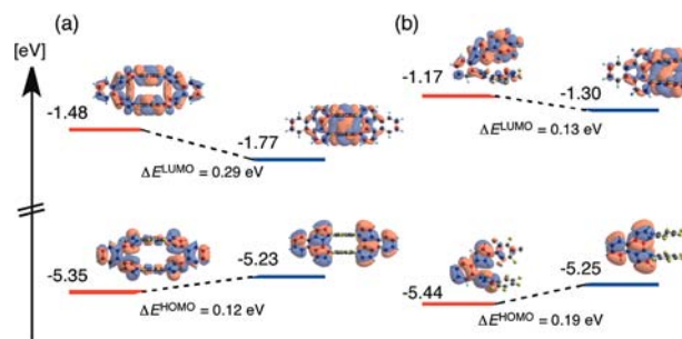
Figure 5. Frontier MO diagrams of (a) 1a , 4a and (b) 2a , 5a calculated at the B3LYP/6-31G(d) level of theory.
