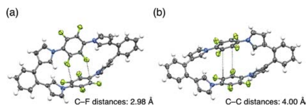
Figure 1. Crystal structures of the two independent conformers of 4a in the unit cell. Thermal ellipsoids are at 50% probability.
